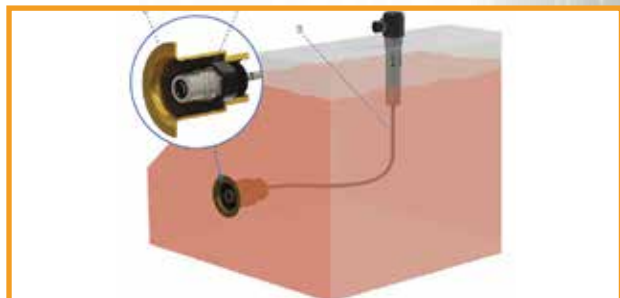
Pressureless Filling
